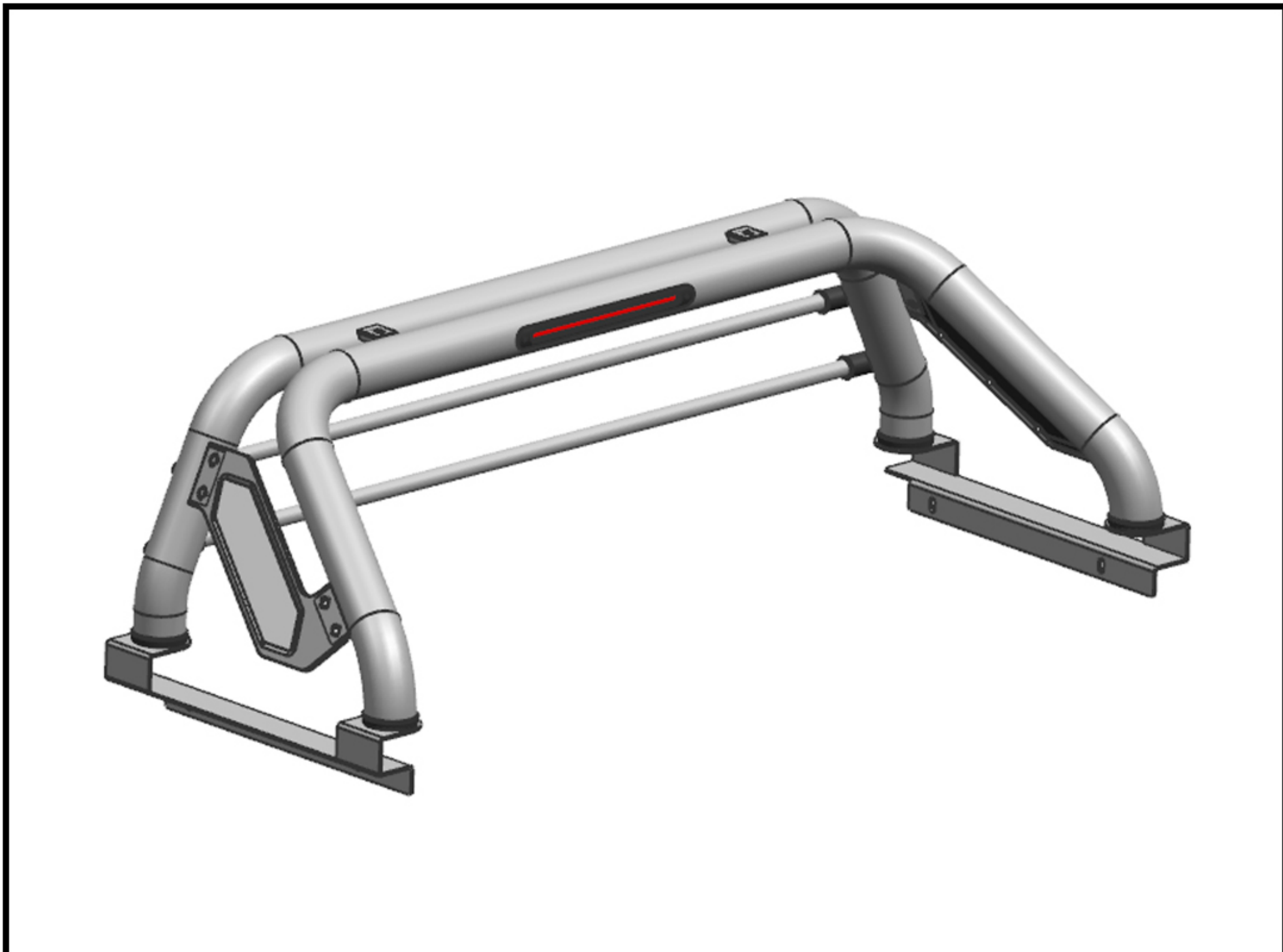
ASSEMBLY DRAWING 1
