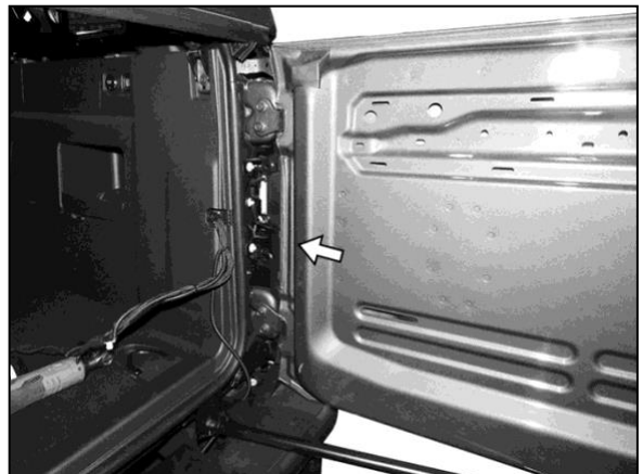
(Fig 4) Remove the plastic cover (arrow). Remove inner wiring harness from rear door
