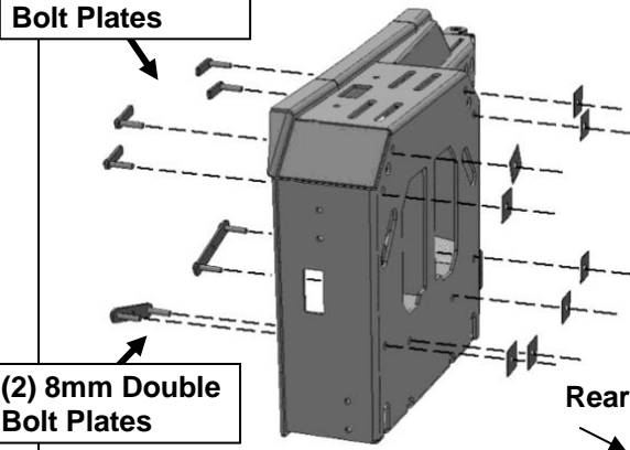
(Fig 8) Insert (4) 8mm Single Bolt Plates through upper mounting holes in the back of the Tire Carrier. Insert (2) 8mm Double Bolt Plates through the lower holes in the Tire Carrier
