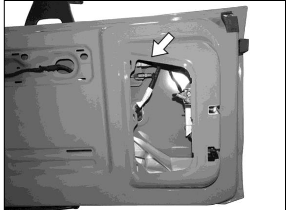
(Fig 2) Disconnect wire harnesses leading to the camera and CHMSL (3rd brake light). Release rubber grommet and pull outer harness through hole in rear door.
