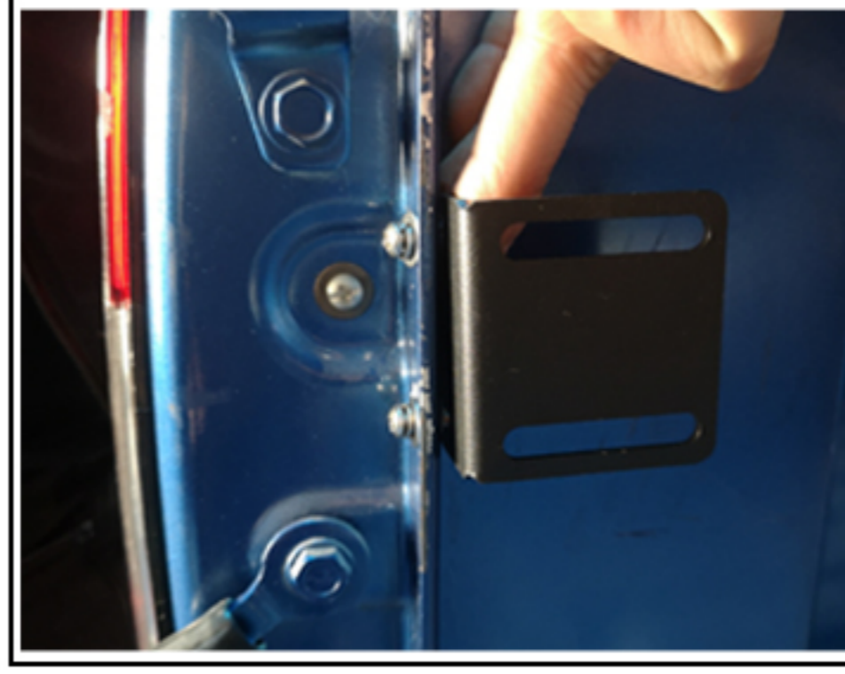
12. Put the bracket 1 into the corresponding hole, insert the screw, and lock it firmly
