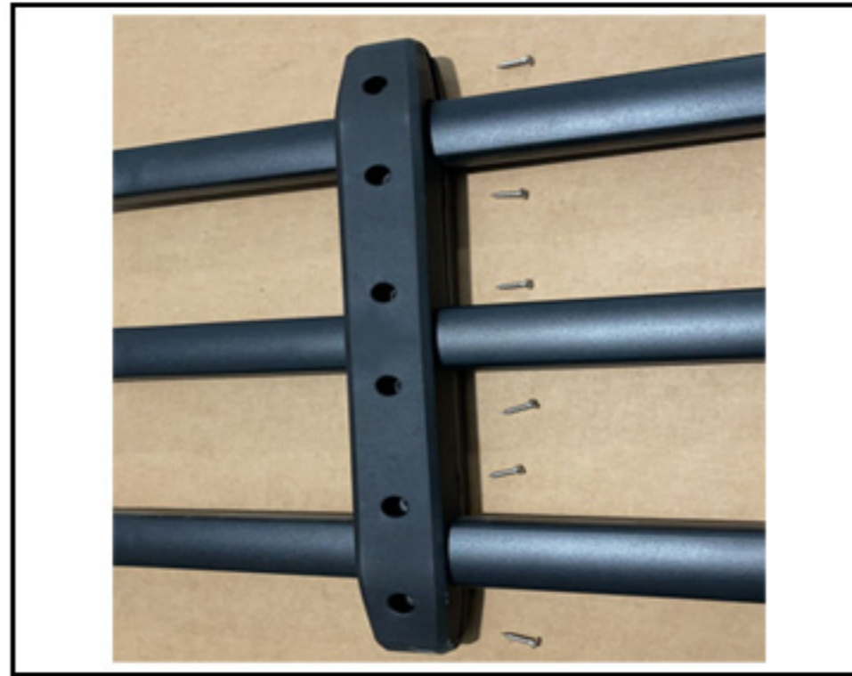
5. Assemble the hole on the other side and lock it with screws
