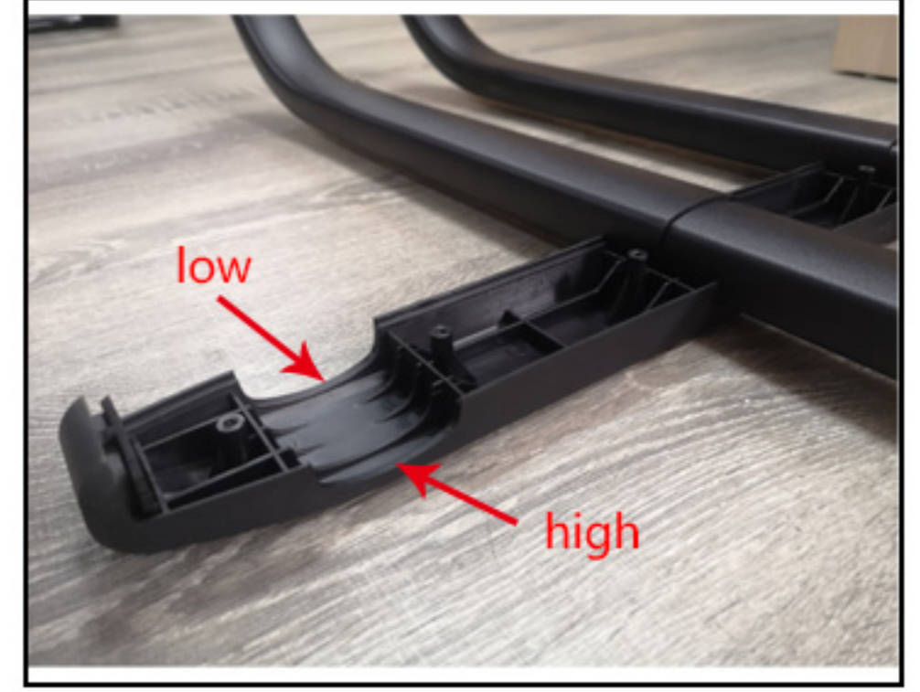
3. As shown in the picture, Place the tube on the bracket, Bracket notches are high or low, the lower side is stuck on the elbow, and the higher side is stuck on the straight pipe
